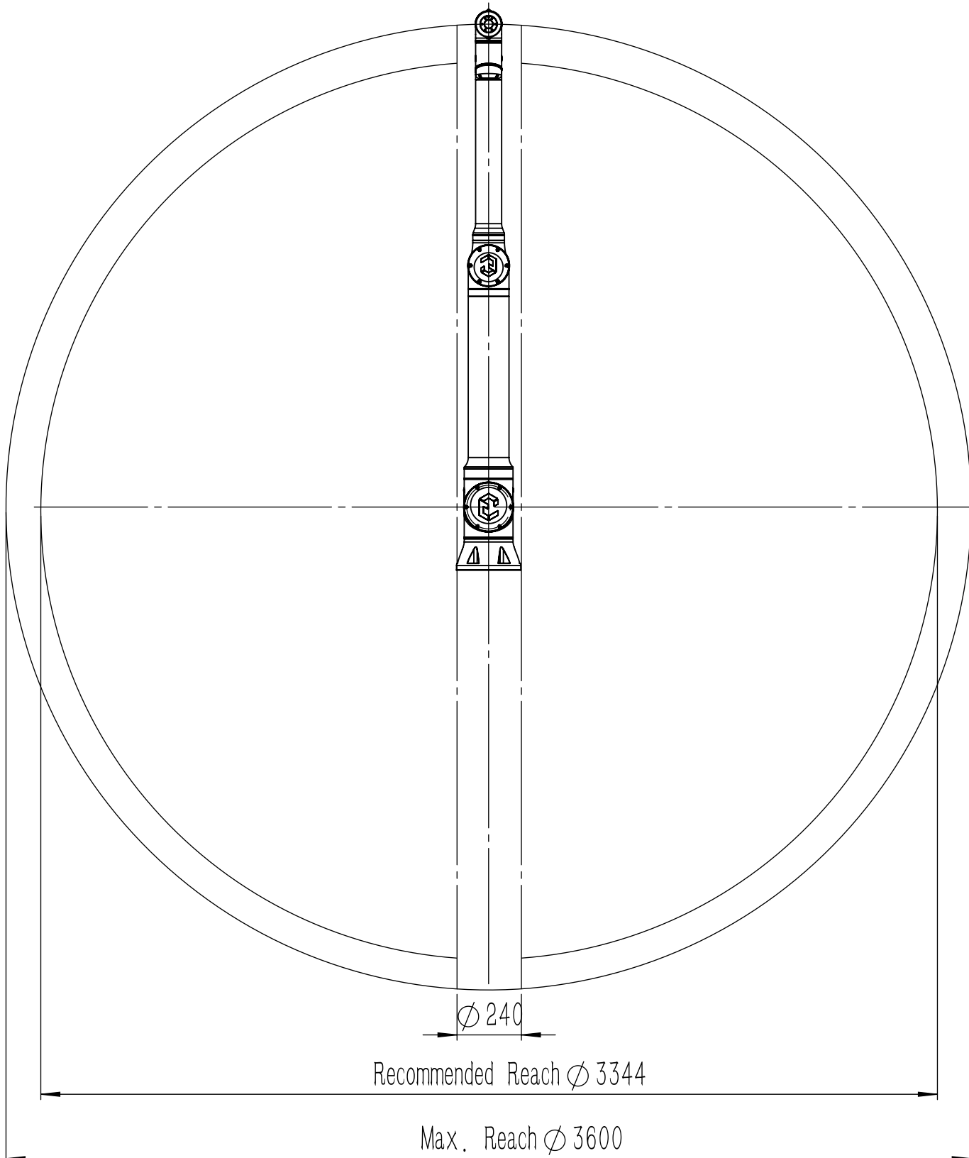
CS620 Working Area Side View
