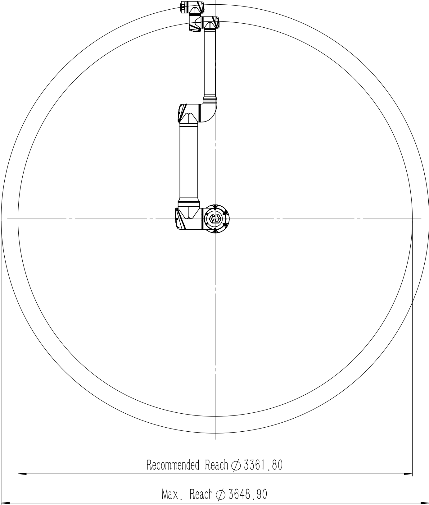
CS620 Working Area Top View
