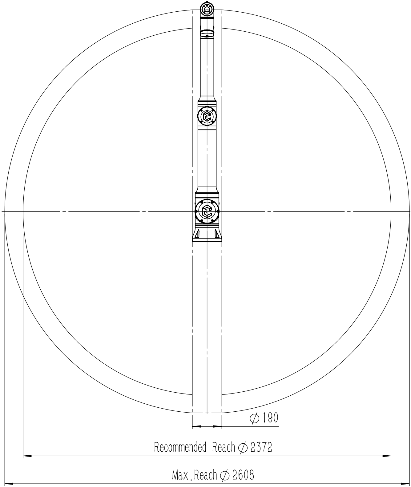
CS612 Working Area Side View
