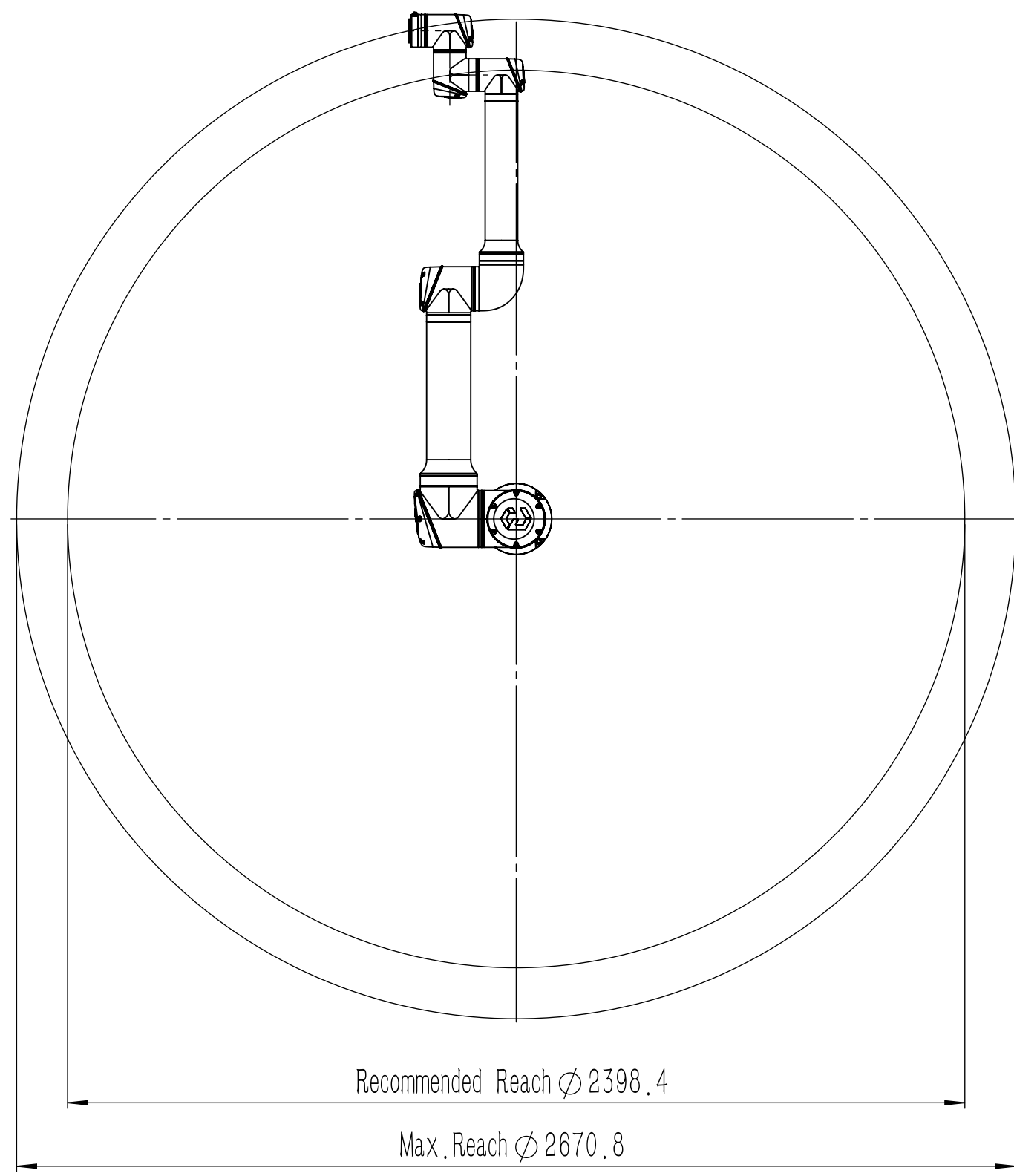
CS612 Working Area Top View
