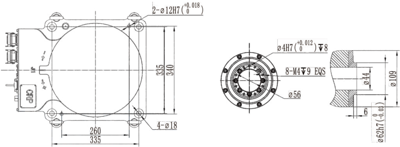
Installation Dimensions of Base
