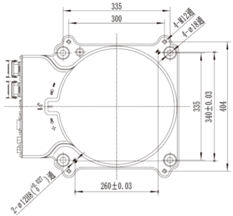
Mounting dimensions of the base
