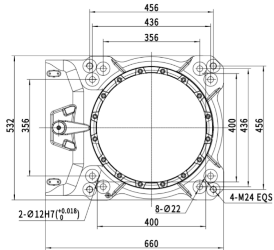
Installation Dimension of Base
