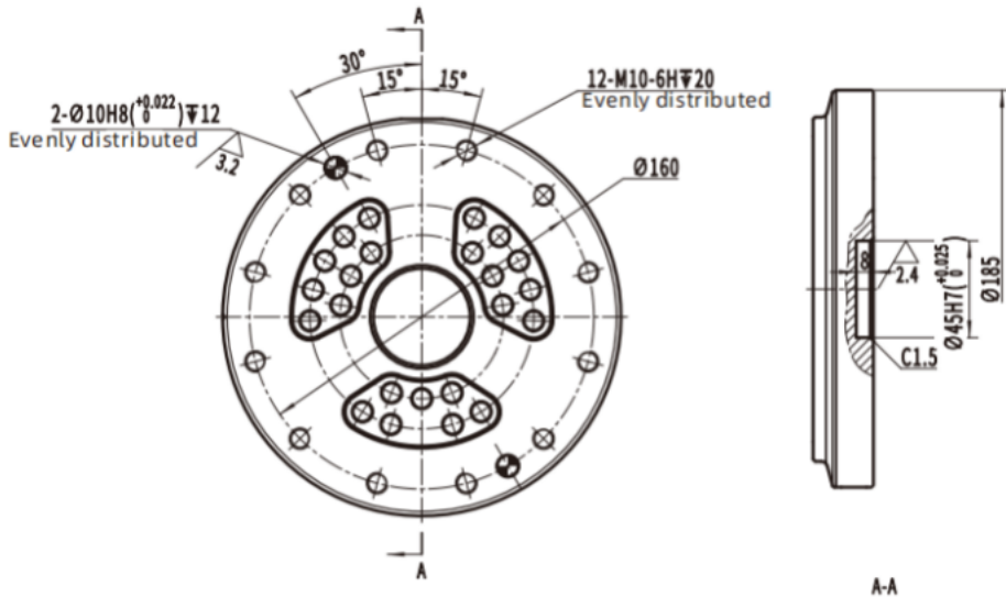
Flange Dimensions
