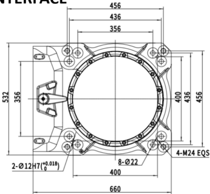
Installation Dimension of Base
