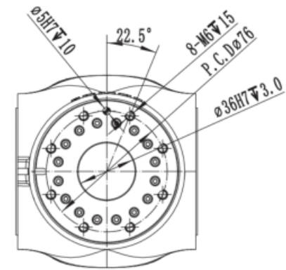
15-12 flange
